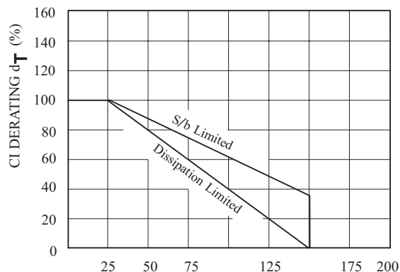
Ic Derating Vs.ccase Temperature
